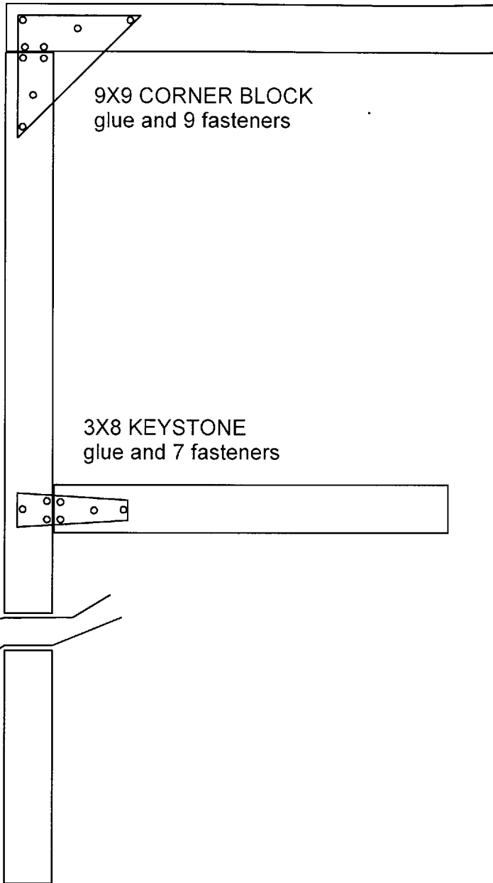
CORNER DETAIL NOT TO SCALE
