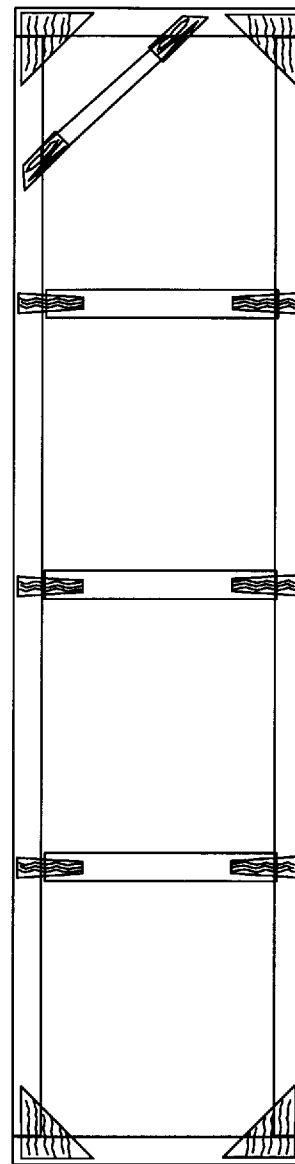
REAR ELEVATION 3'X12' FLAT SCALE 1/2"=1'
